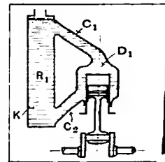
Fig. 5—Diagram of thermo-siphon system. R_1 , reservoir. K , radiator. C_1 , water outlet. C_2 , water inlet. D_1 , water jacket.
